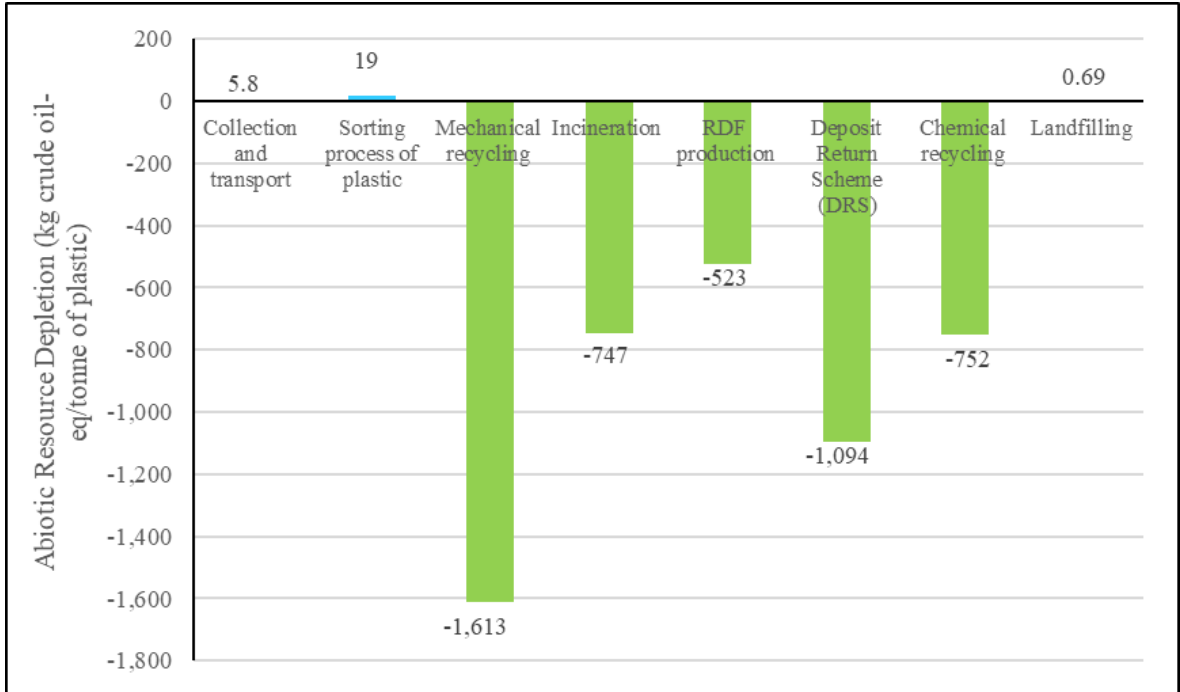
Figure 7.5. Abiotic Resource Depletion/Savings Potential from All Kinds of Plastic Treatment Options
