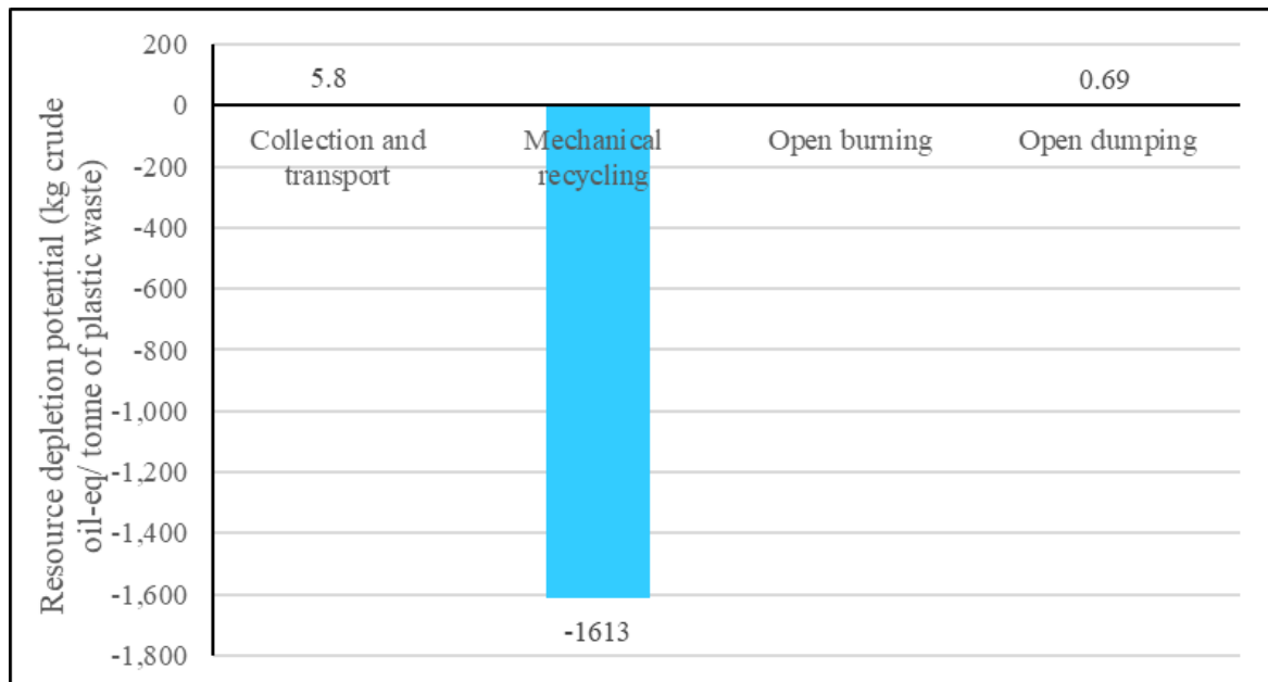
Figure 7.2. Abiotic Resource Depletion Potential/Savings from Existing Plastic Waste Management in ASEAN
